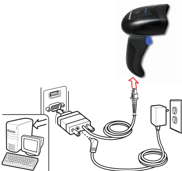
Figure 3. RS-232 Connection
